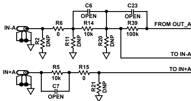
FIGURE 3. INPUT STAGE
