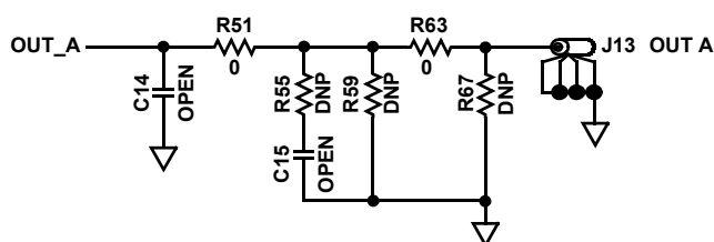
FIGURE 4. OUTPUT STAGE
